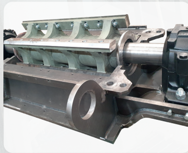
Heavy duty rotor.
